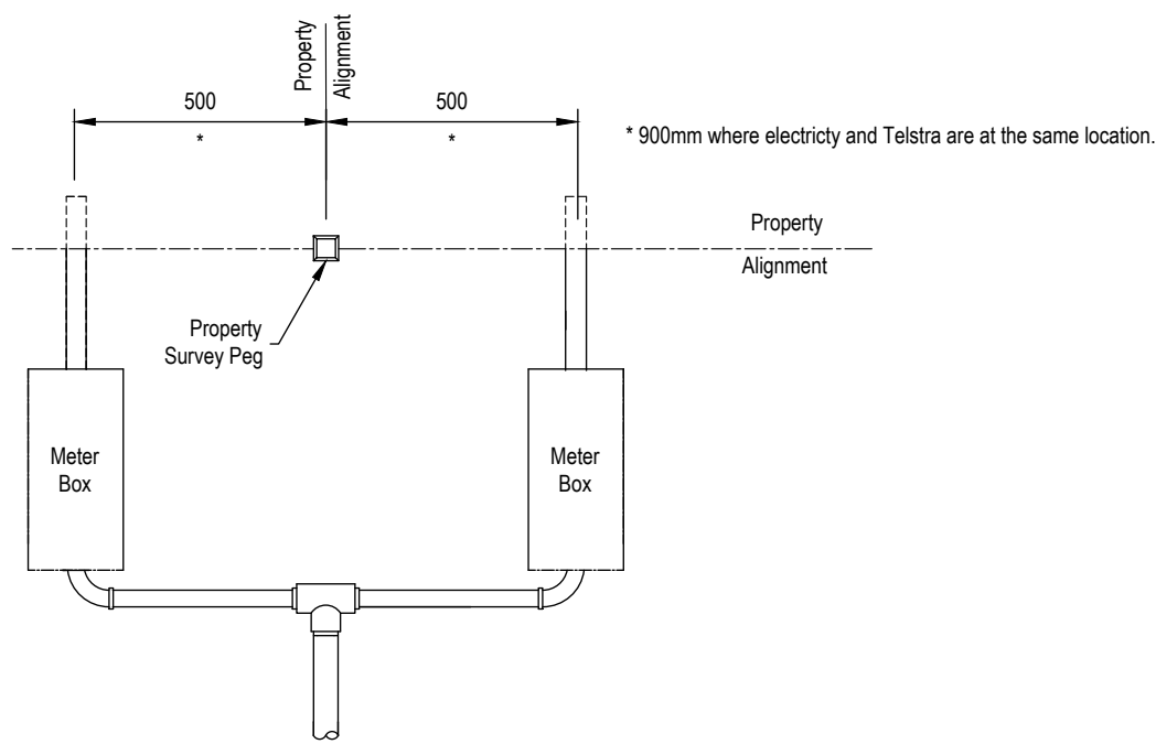
METER BOX DETAIL AT PROPERTY LINE
