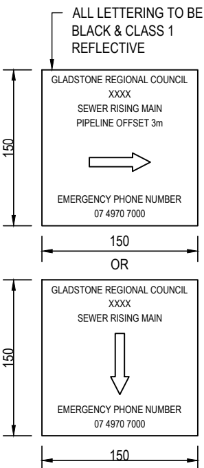
SIGNAGE PLATE DETAILS NOT TO SCALE
