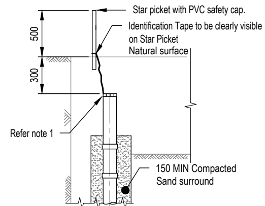
VERTICAL H.C. BRANCH PRE SITE DEVELOPMENT DETAIL N.T.S.
