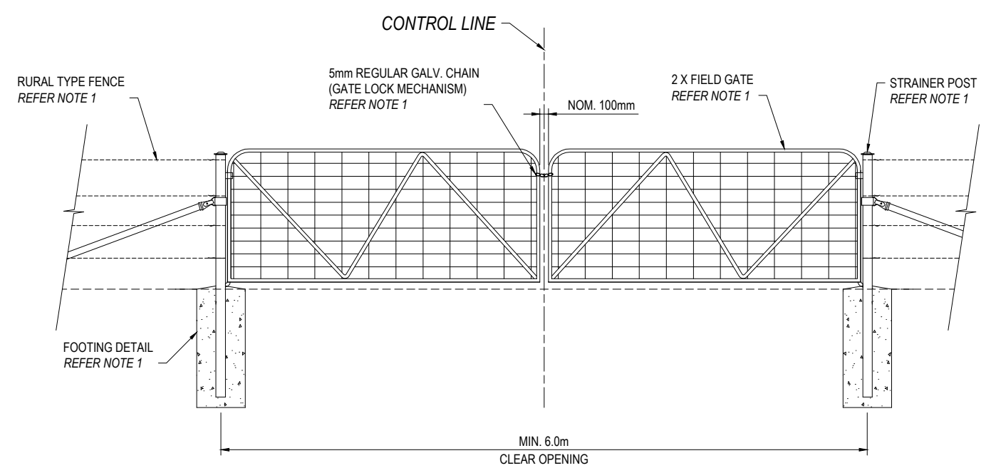
STANDARD GATE DETAIL 1:25
