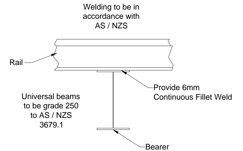
WELDING DETAIL
