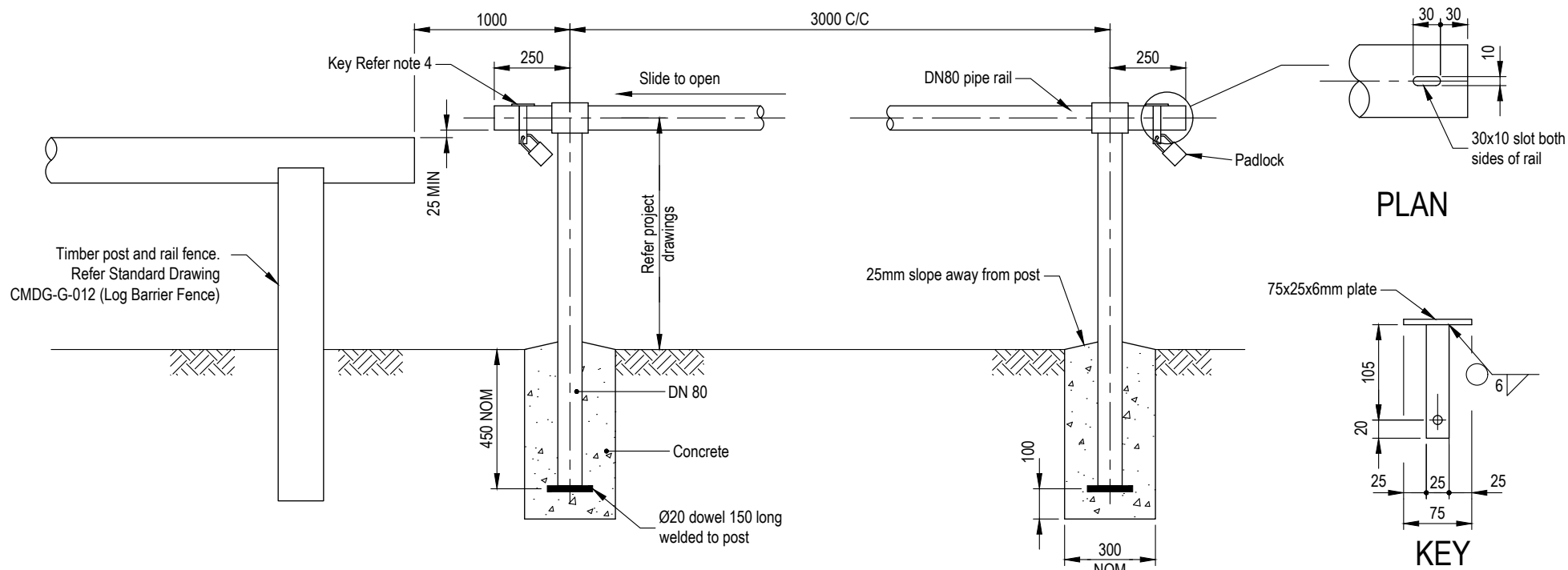
ELEVATION LOCKING RAIL TYPE 1
