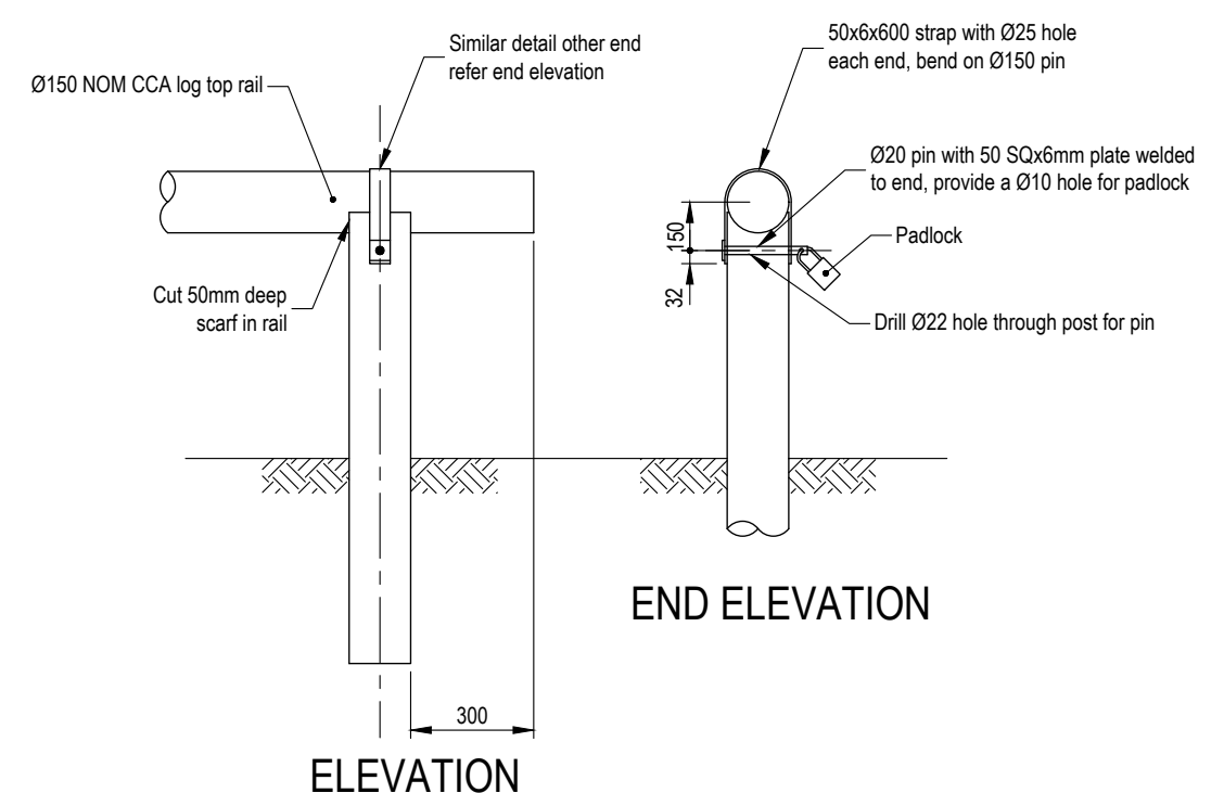
LOCKING RAIL TYPE 2
