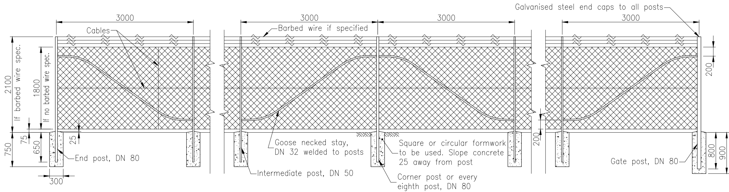
TYPICAL SECTION
