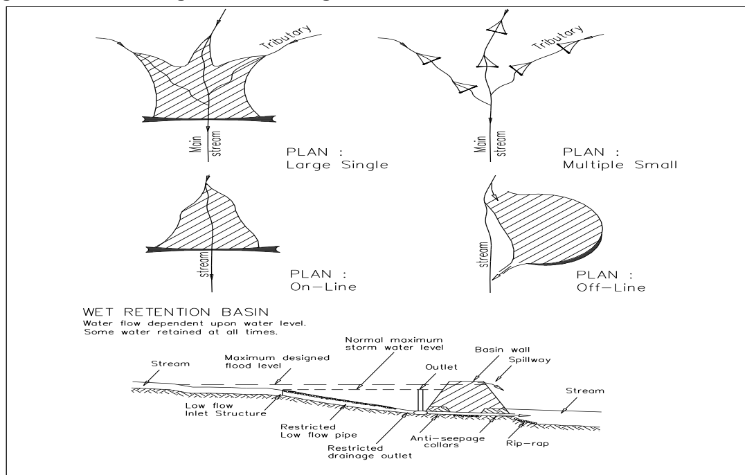
Figure D07. 18.1 - Configuration and Design of Wet Retention Basins
