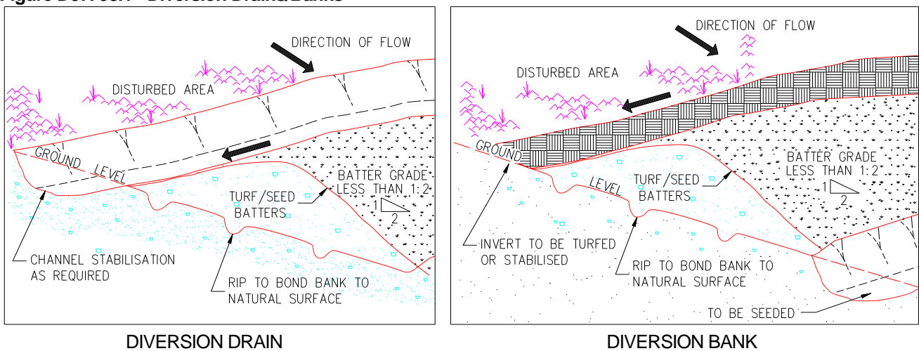
Figure D07.08.1 - Diversion Drains/Banks
