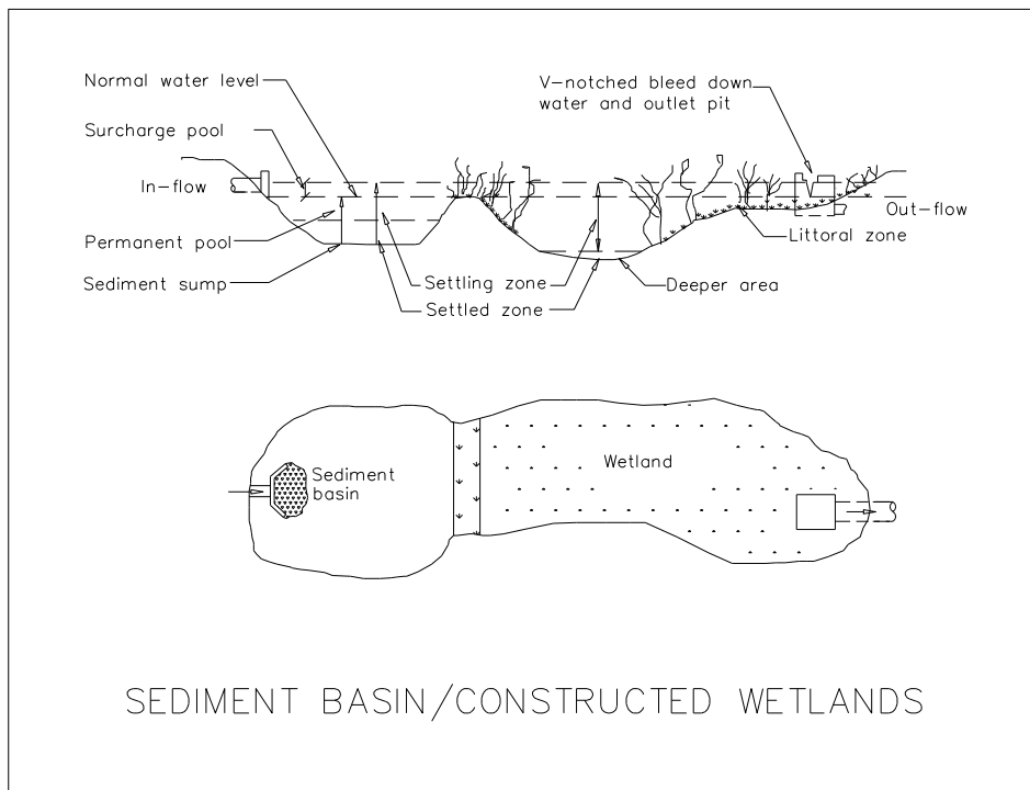
Figure D07. 21.1 - Sediment Trap/Constructed Wetland
