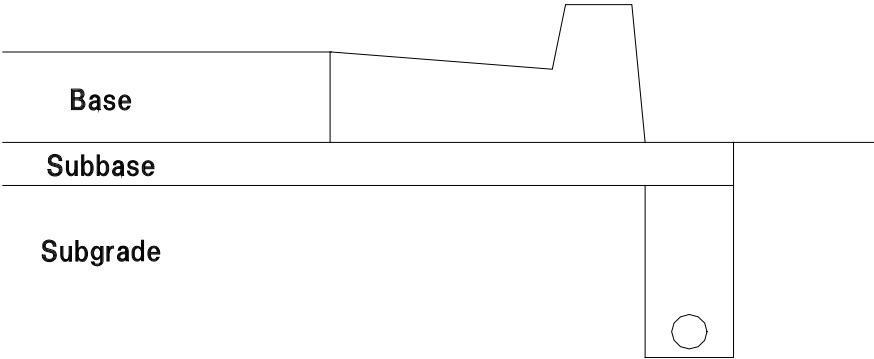
Figure D04. 06.1 - Typical Subsoil Drain
