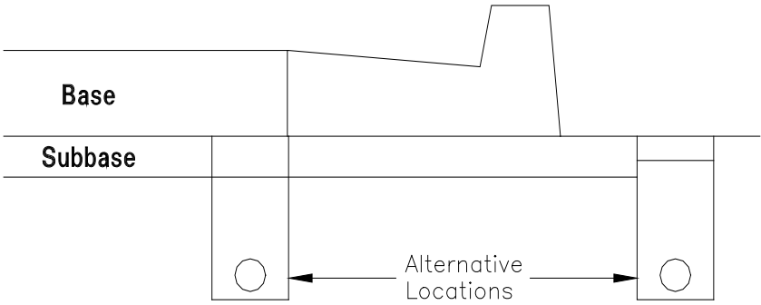
Figure D04. 06.2 - Typical Sub-pavement Drain
